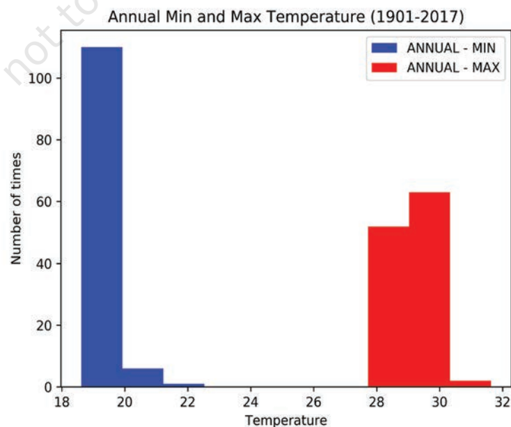
Figure 4.12: Histogram for 'ANNUAL - MIN'
