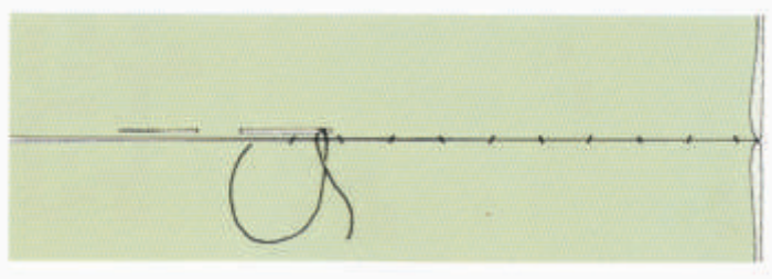
Even Slip stitch
