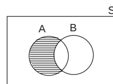
Shaded portion is A - B = A \cap B'
