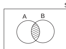
Shaded portion is A \cap B
