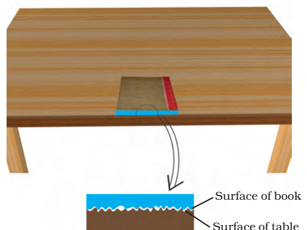
Fig. 12.5 : Surface irregularities
